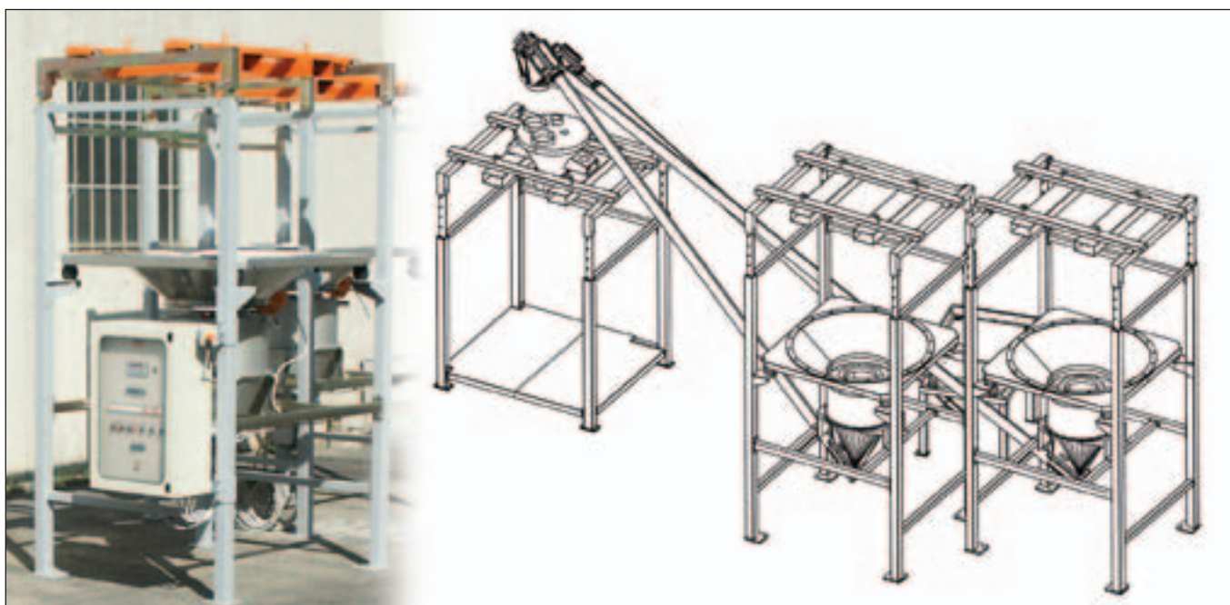
Plant for Bulk Bag - hopper with micro-components unloading and subsequent batching directly in the Bulk Bag filling station on loading cells
